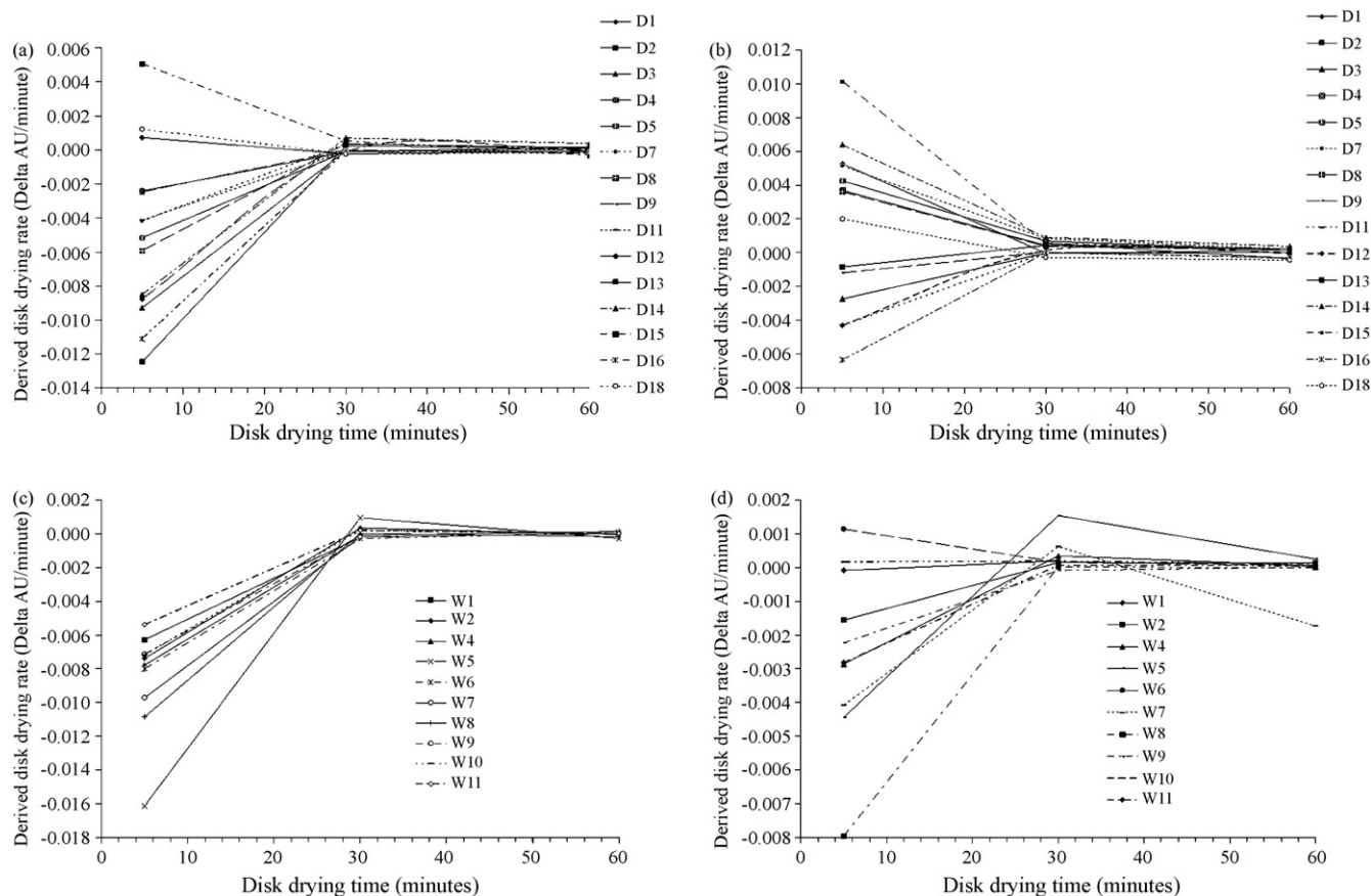
Fig. 8. Apparent disk drying rate curves derived from absorbance data at THz bands around 54 and 210 \text{cm}^{-1} : (a) DC tablets at 54 \text{cm}^{-1} ; (b) DC tablets at 210 \text{cm}^{-1} ; (c) WG tablets at 54 \text{cm}^{-1} ; (d) WG tablets at 210 \text{cm}^{-1} .
