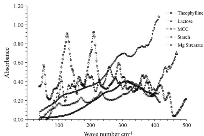
Fig. 2. Uncorrected raw THz spectra of pure pharmaceutical tablet components.
